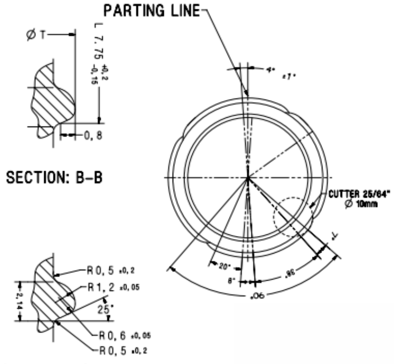
CUTTER PROFILE
